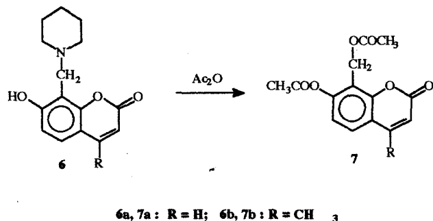
Figure 2. Diacetyl derivative.
